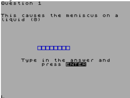
Physics
