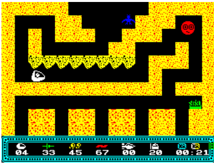
The Planets
